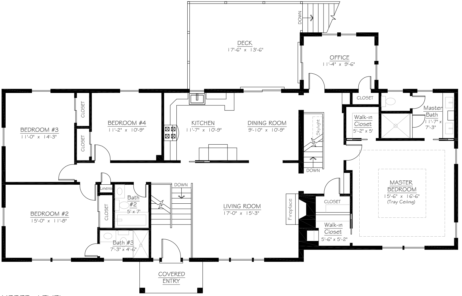
UPPER LEVEL 3812 Chantal Lane
